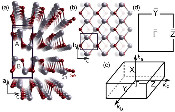
FIG. 1. The crystal structure of SnSe viewed (a) along, and (b) perpendicular to the layers. The lower of the two layers contained in the unit cell, A and B , has in panel (b) been made nearly invisible. The unit cell size is 11.5 \times 4.2 \times 4.4 \text{ \AA}^3 . The reciprocal space repetition cells: (c) the three-dimensional bulk Brillouin zone with \Gamma X = 0.27 \text{ \AA}^{-1} , \Gamma Y = 0.75 \text{ \AA}^{-1} , \Gamma Z = 0.71 \text{ \AA}^{-1} ; (d) the layer-bound two-dimensional surface Brillouin zone. The points Y and Z project along the a direction into \bar{Y} and \bar{Z} , respectively.
